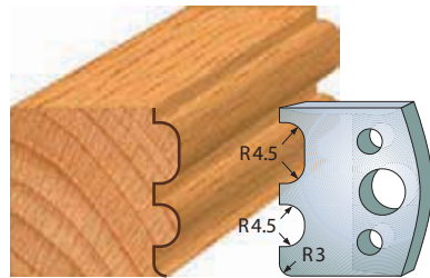
Pair of knives 690.007 Pair of limiters 691.007
